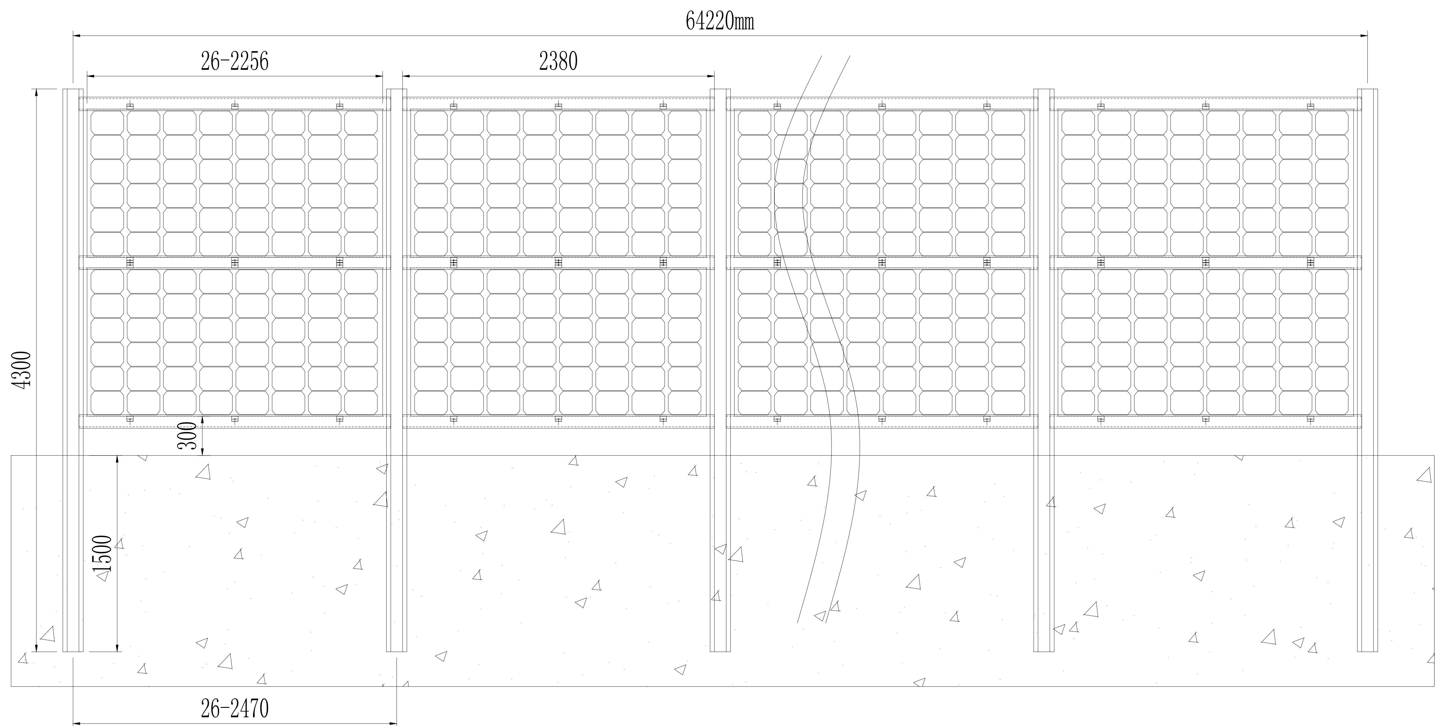
2*26 Top View Total: 30 Sets (1560pcs)
